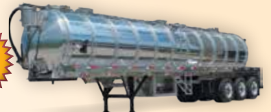
7000 - 9000 Gal. Aluminum Tri-Axle Trailers | Air ride suspension (tri-axle), pump platform, bright finish, LED lights, Betts valves.
