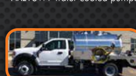
(13961) NEW Imperial 1300 U.S. gallon, portable toilet service unit mounted on a 2021 Ford F550 cab and chassis with a Masport HXL4 pump package.
