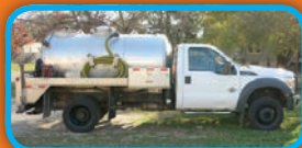
(4246V) 2012 Ford F550 cab & chassis with an Imperial 1,100 U.S. gal.s, 3 compartment 150/600/350 Aluminum portable toilet service unit, with a Masport HXL4 vacuum pump.
