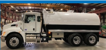
2020 Kenworth T370 , 3,600-gallon 1/4" powder-coated steel vacuum tank, Jurop LC420 pump, hose trays, 36" rear hatch, heavy duty bumper, (2) 4" suction ports, trailer hookups, (2) 36" toolbox. 350hp Cummins, Allison auto transmission, chrome bumper, aluminum wheels. .... $132,866
