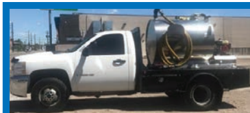
2009 Chevy 3500HD , Duramax, Allison auto., 4WD. NEW aluminum 300 waste/150 fresh vacuum tank, HXL2 Masport pump, washdown system.
