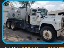
(1165C) 1984 Mack R686ST with a 1999 Keith Huber Dominator 3000 carbon steel, dump type, DOT, vacuum tank unit.
