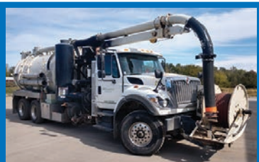
2012 GapVax MC1510 w/hydroexcavation, Allison automatic transmission, Giant jetting pump, Giant hydro pump, 18" blower, new tires. International remanufactured engine 2019. Ready to work. ....$190,000 OBO
