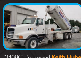
(3408C) Pre-owned Keith Huber Dominator , 4,000 U.S. gal., two compartment, dump type unit, with a Becker 440 vacuum pump package. Mounted on a 1999 Sterling cab & chassis.
