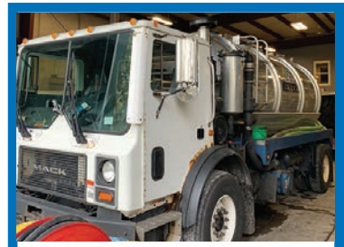
2004 Mack MR cab-over bulk hauler. Liquid automatic transmission, 20,000 lbs. front axle, 30,000 lbs. rear axle. GVW - 49,000 lbs. 3,000-gallon capacity aluminum tank, Gardner Denver RFL 80 PTO pump - less than 500 hours on rebuilt pump. .... $63,500
