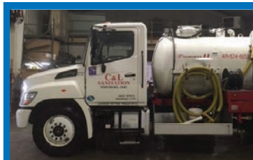
2012 Hino 268 auto/air with Keith Huber Princess 1,200-gallon waste/350-gallon water, Masport HXL75 vacuum pump, PTO HotShift, Burks DC10 water pump, 2-unit carrier. Clean cab. 120,000 miles. $39,000 419-466-1349, OH P01
