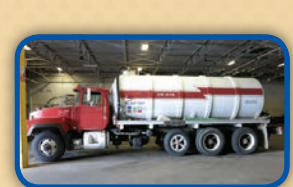
(3130V) 1997 Mack RD688S Tri-Axle cab & chassis with a 4,500 gal. aluminum vacuum tank and Wittig RFL100 pump package.
