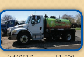
(4468C) Pre-owned 1,500 U.S. gal., carbon steel, vacuum pressure tank. Mounted on Freightliner M-2 cab and chassis with a Masport HXL400WV vacuum pressure pump.
