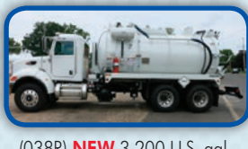
(038R) NEW 3,200 U.S. gal. , carbon steel, D.O.T. certified 412 vacuum tank; dump type with full open rear door and a Presvac PVB 750 vacuum-pressure pump installed on a 2015 Peterbilt 348 cab and chassis.
