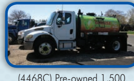
(4468C) Pre-owned 1,500 U.S. gal., carbon steel, vacuum pressure tank. Mounted on Freightliner M-2 cab and chassis with a Masport HXL400WW vacuum pressure pump.
