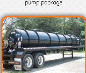
(3901C) 2012 Dragon 5,460 U.S. gallon, Steel, vacuum tank trailer.
