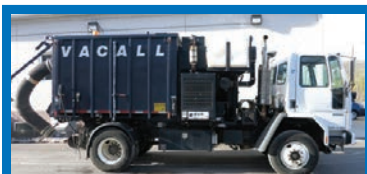
Pre-owned Vacall Model VC13 catch basin cleaning unit mounted on a 2006 Sterling SC8000 cab & chassis. (Stock# 1536V) www.VacuumSalesInc.com (888) VAC-UNIT (822-8648) PBM
