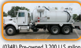
(034R) Pre-owned 3,200 U.S. gallon, carbon steel, D.O.T. certified 412 vacuum tank; dump type with full open rear door and a Presvac PVB 750 vacuum-pressure pump installed on a 2014 Peterbilt 348 cab and chassis .
