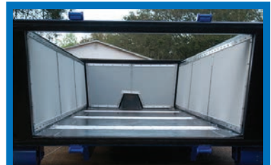
New 2016 20-yard and 15-yard de-watering filter boxes "Vacuum Truck Special", including roll-over tarp system, permanent filter material, loading manifold, drain and wash-out ports. 20-yard: $24,500. 15-yard: $22,500. For more information call
