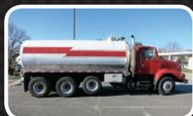
(9982V) 2000 International 2674 triaxle with 4000 waste—200 water and Wittig RFL100 vacuum pump and Harben jet pump system.
