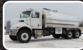
(13670V) New 4,000 U.S. gallon, aluminum, vacuum-pressure tank. Mounted on 2016 Peterbilt 348 cab and chassis with a Masport HXL400WV vacuum pressure pump package.
