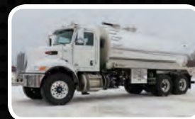
(13670V) New 4,000 U.S. gallon, aluminum, vacuum-pressure tank. Mounted on 2016 Peterbilt 348 cab and chassis with a Masport HXL400VV vacuum pressure pump package.
