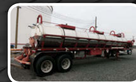
(5006V) 1990 Presvac 5,500 gallon stainless steel vacuum tank trailer with a Presvac PV750 vacuum pressure pump and engine package
