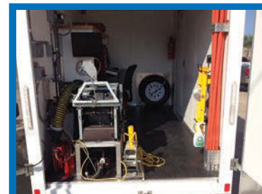
Aries Mainline Camera System: Dealer demo. Pathfinder Series zoom camera and tractor for 6"-24" lines. Generator, wash-down system, 1,000 ft. cable. Saturn control unit. Luxury trailer, full wheel kit. .... $55,000
