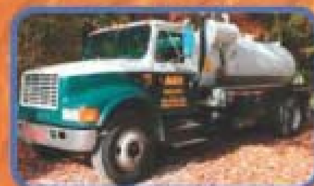
(2282V) 1999 International 4700 Cab and chassis with a pre-owned 3 - compartment Coleman 600, 250, 100, stainless steel vacuum tank with a Masport vacuum.
